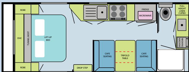
OPAL C19'6" x 7'9" - MD
