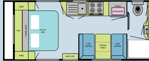
OPAL C17'6" x 7'9" - MD - SINGLE AXLE
